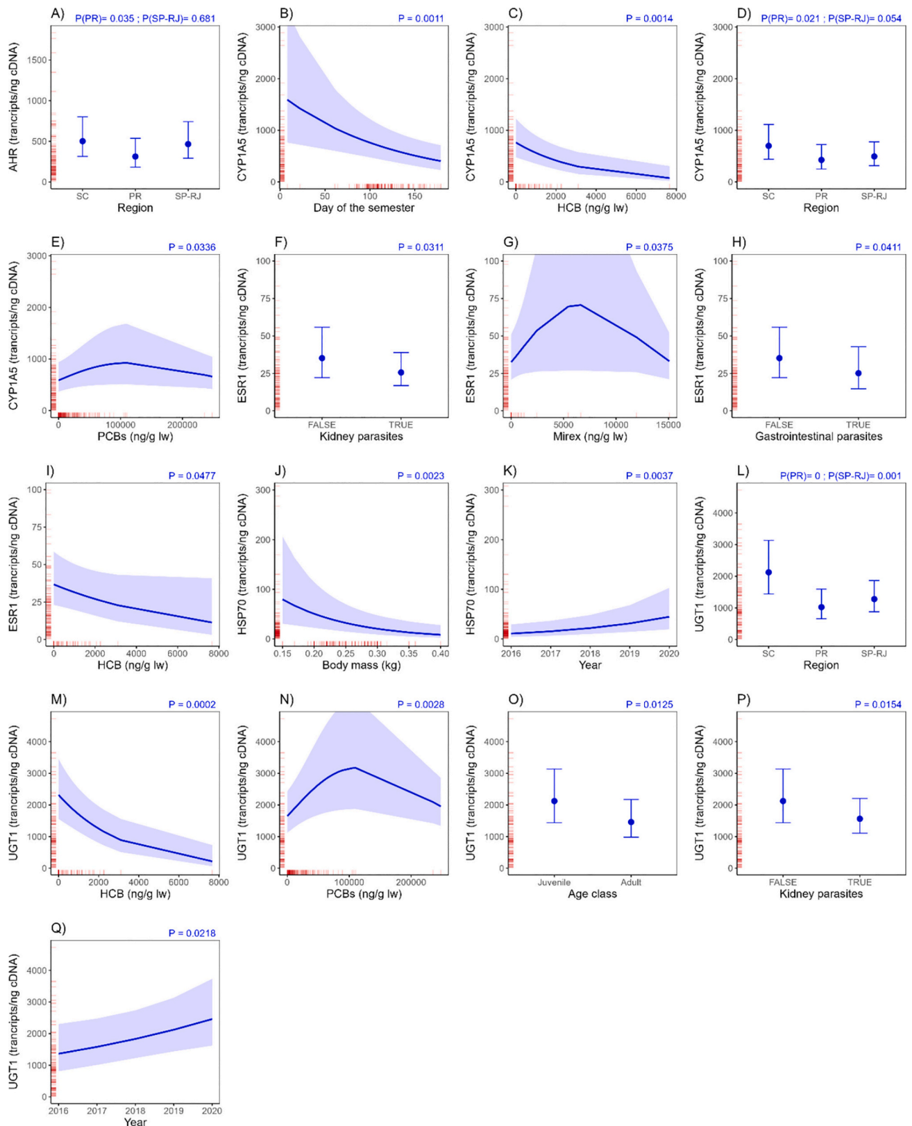
Fig. 3. Effects plots for significant variables ( p < 0.05 ) in General Additive Models (GAM) for the liver transcription levels of aryl hydrocarbon receptor ( AhR ), cytochrome P450 1A5 ( CYP1A5 ), estrogen receptor alpha 1 ( ESR1 ), heat shock protein 70 ( HSP70 ) and UDP-glucuronosyl-transferase ( UGT1 ) genes in Manx shearwaters ( Puffinus puffinus ) stranded along the southern and southeastern coast of Brazil. Blue lines or circles represent the model predictions, with their 95 % confidence intervals represented by shaded blue areas or blue error bars. Red rugs along the margins of the plots represent the data distribution used to produce the model. (For interpretation of the references to colour in this figure legend, the reader is referred to the web version of this article.)
