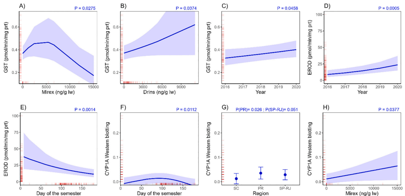
Fig. 2. Effect plots for significant variables ( p < 0.05 ) in General Additive Models (GAM) for the liver enzymatic activity of glutathione S -transferase (GST) and 7-ethoxyresorufin O -deethylase (EROD) and the immunodetection level of the cytochrome P450 1A proteins (CYP1A) in Manx shearwaters ( Puffinus puffinus ) stranded along the southern and southeastern coast of Brazil. Blue lines or circles represent the model predictions, with their 95 % confidence intervals represented by shaded blue areas or blue error bars. Red rugs along the margins of the plots represent the data distribution used to generate the model. (For interpretation of the references to colour in this figure legend, the reader is referred to the web version of this article.)
